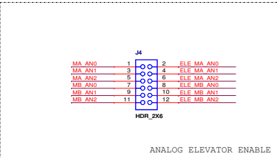
ANALOG ELEVATOR ENABLE
