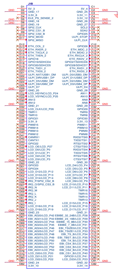
PCI EXPRESS X 16 DUMMY PORT
