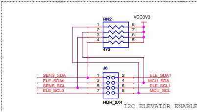
I2C ELEVATOR ENABLE
