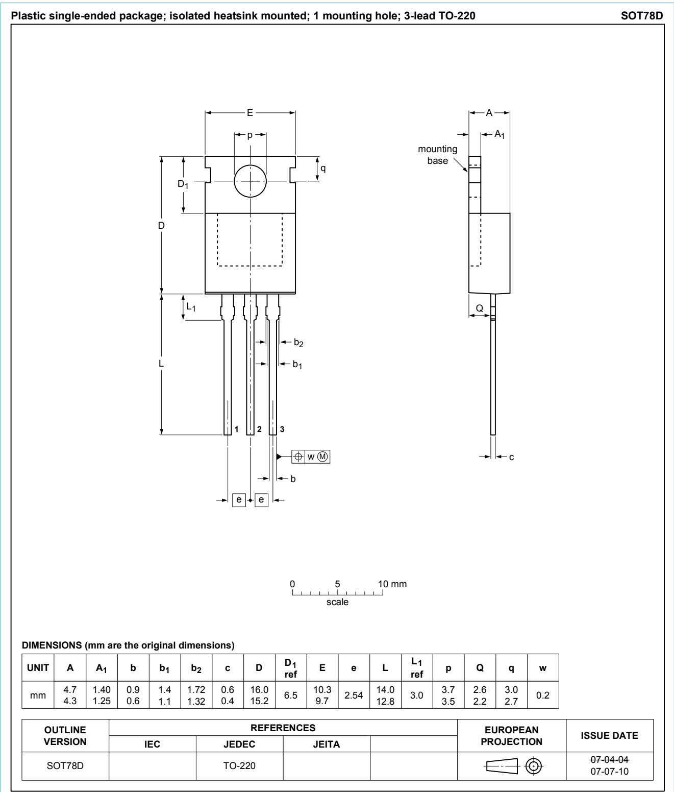
Fig. 1. Package outline TO-220AB (SOT78D)
