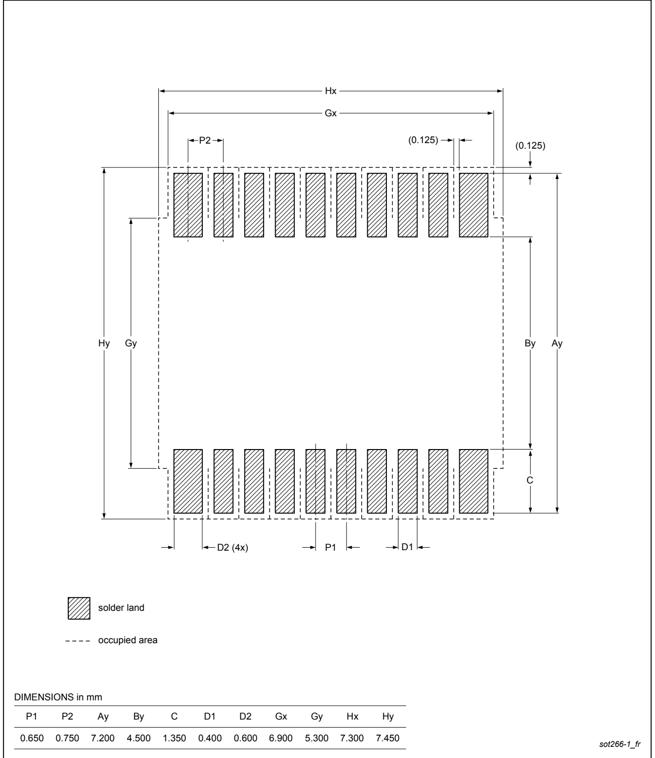
Fig. 2. Reflow soldering footprint for SSOP20 (SOT266-1)
