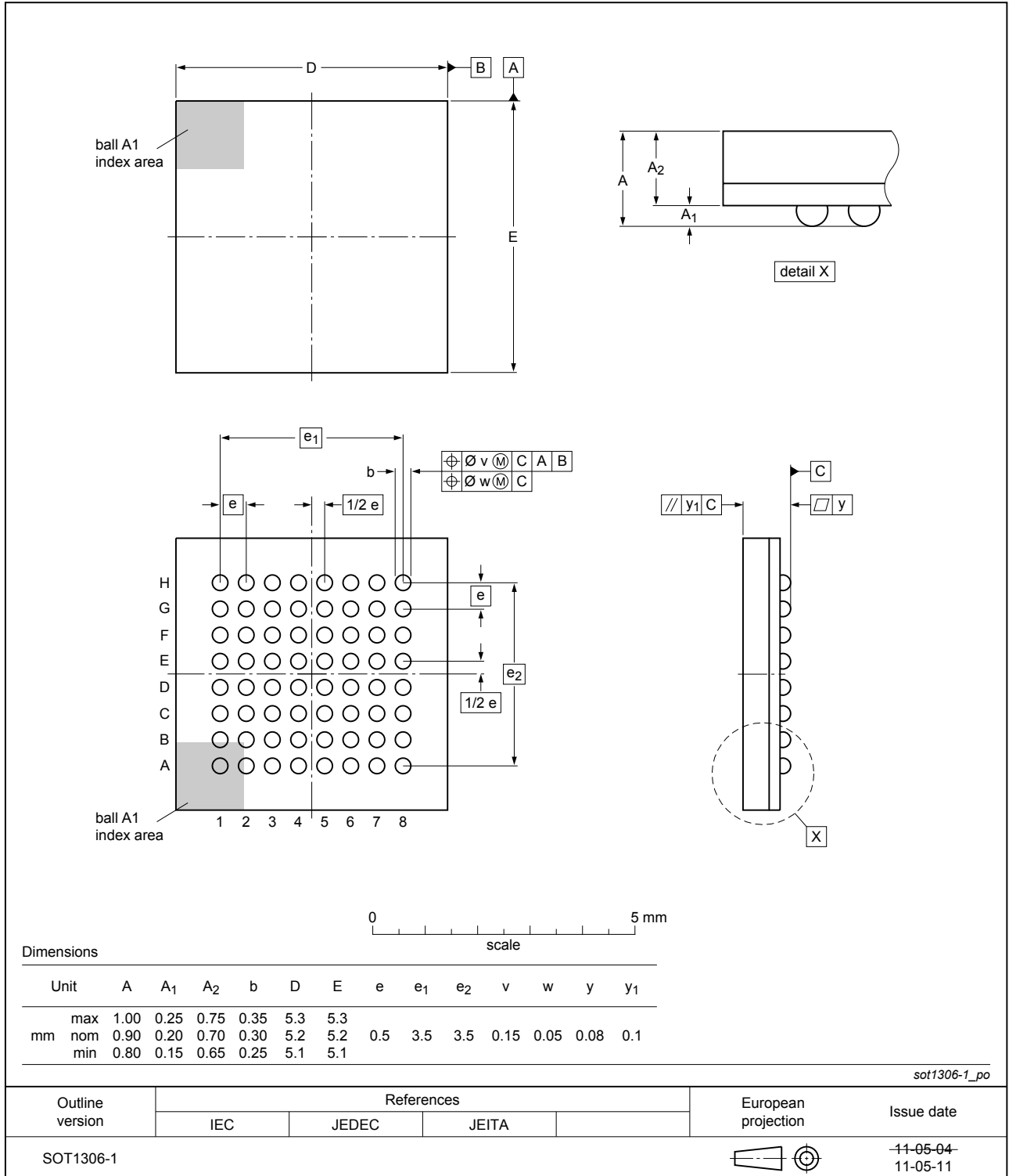
Fig. 1. Package outline VFBGA64 (SOT1306-1)
