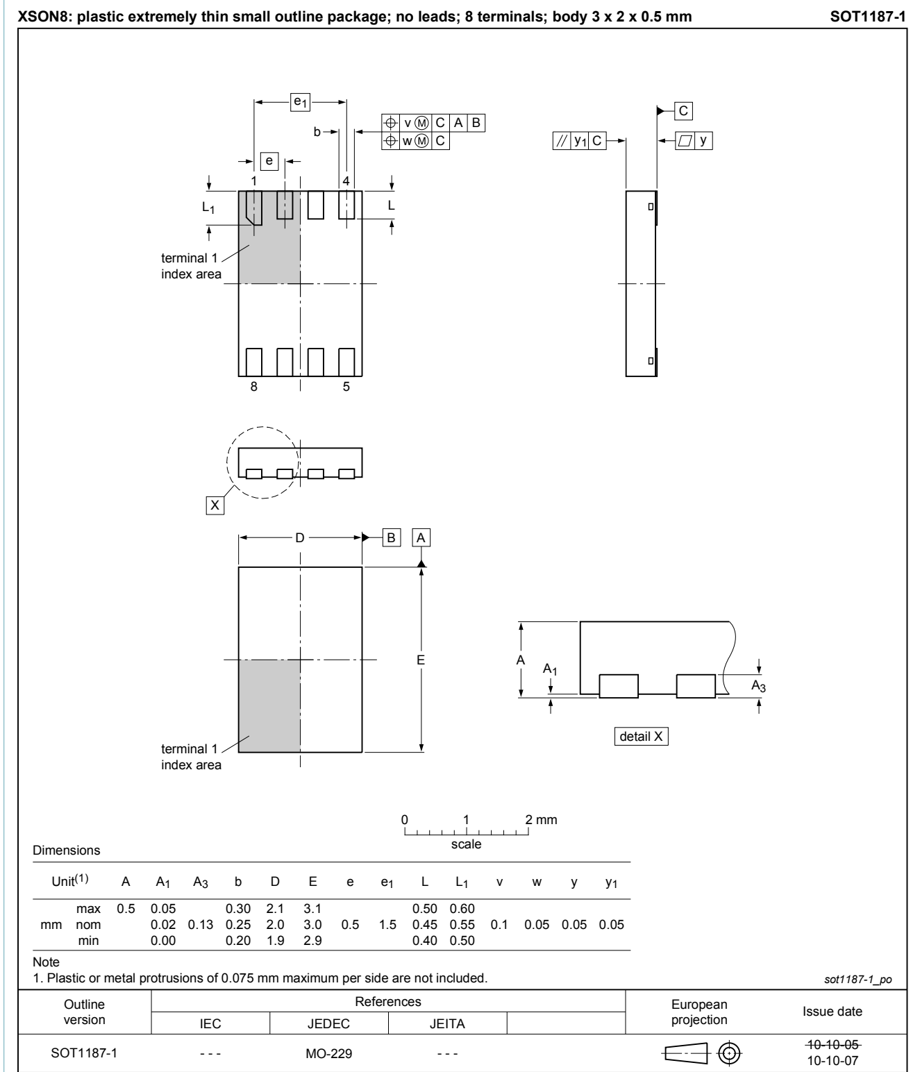
Fig. 1. Package outline XSON8 (SOT1187-1)
